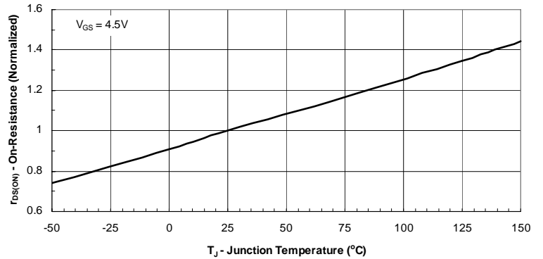
On-Resistance vs. Junction Temperature
